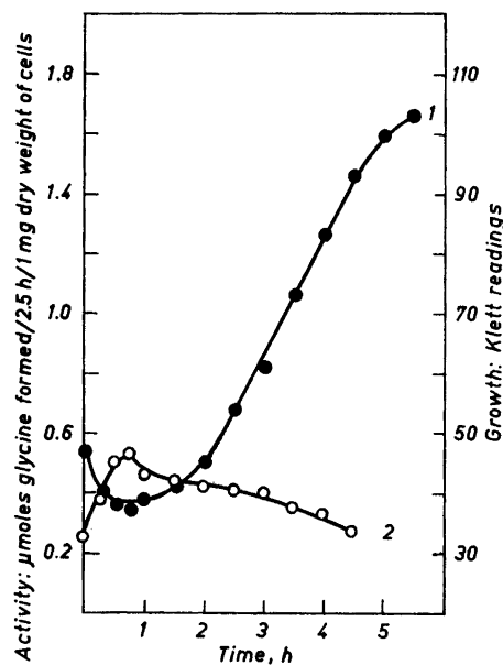
Fig. 10. Serine hydroxymethyltransferase activity during the growth of Str KQGly . 1. Growth curve. 2. Activity curve.
