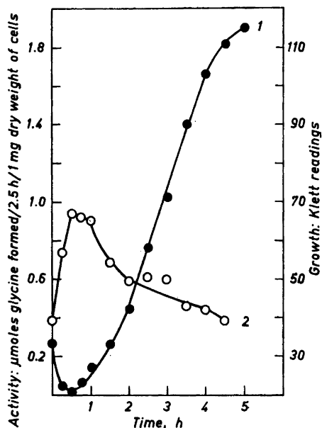
Fig. 9. Serine hydroxymethyltransferase activity during the growth of Str KQ . 1. Growth curve. 2. Activity curve.
