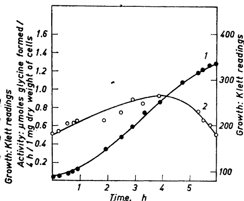
Fig. 8. Serine hydroxymethyltransferase activity during the growth of Lb. arabinosus 17-5. 1. Growth curve. 2. Activity curve.
