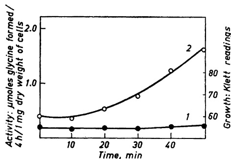
Fig. 3. Serine hydroxymethyltransferase activity during the lag phase of E. coli . 1. Growth curve. 2. Activity curve.
